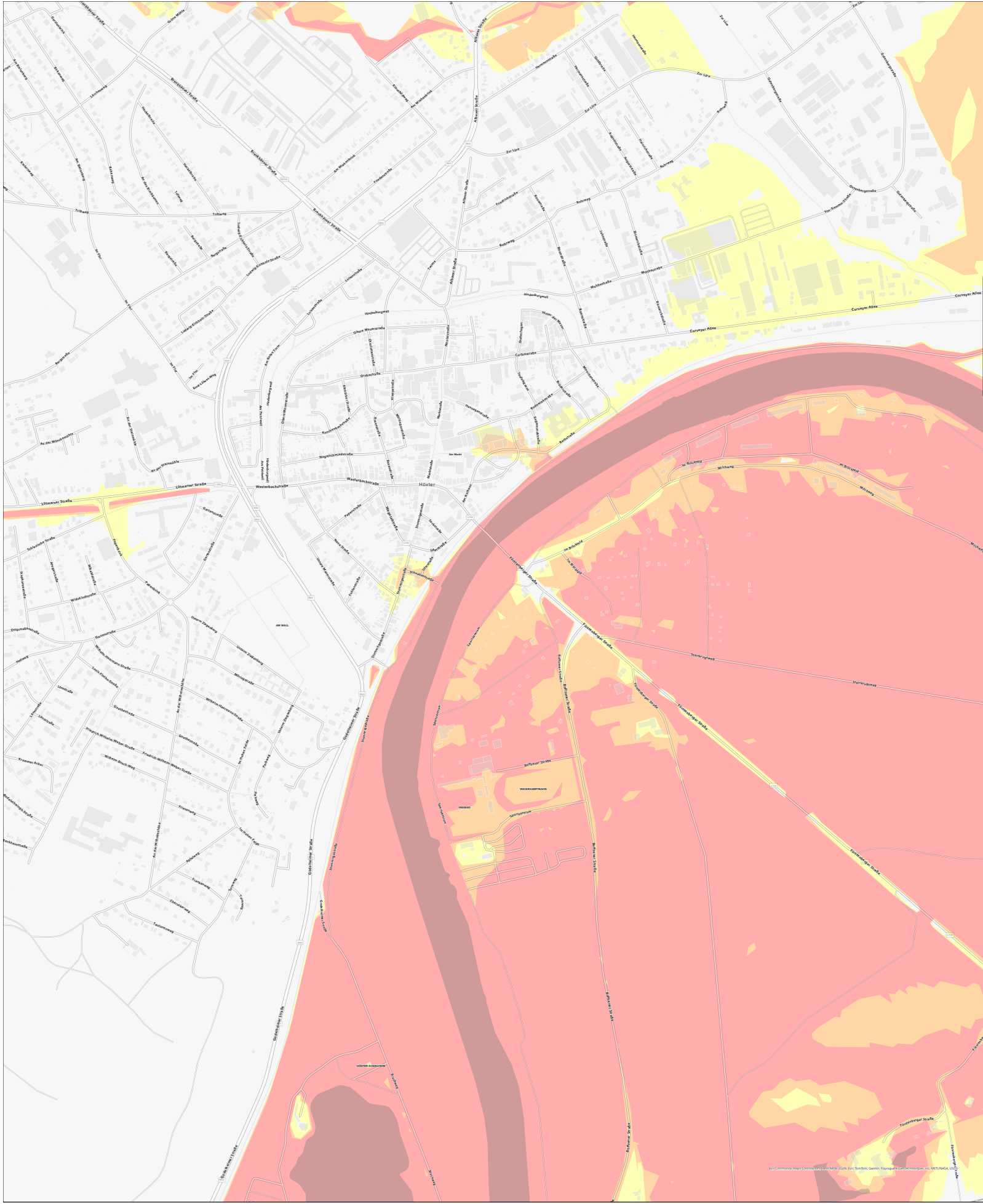
Flood Simulation
